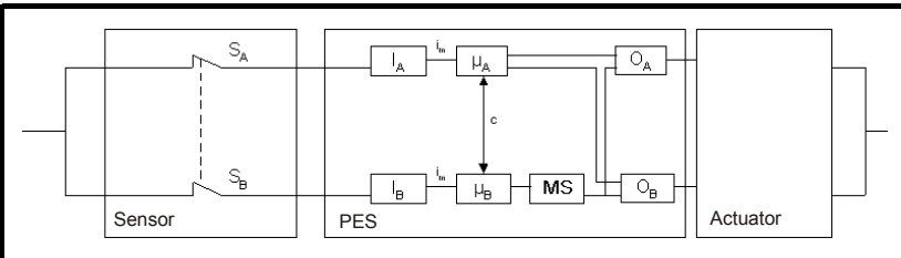
Figure 3-3 Grouped inputs
