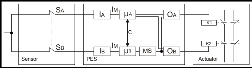
Figure 4-1 Signal processing in two channels
